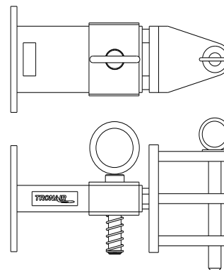
FIGURE 3 01-1950-5000 Standard Telecoupler
