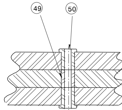
SECTION VIEW OF SHEAR PIN BUSHINGS
