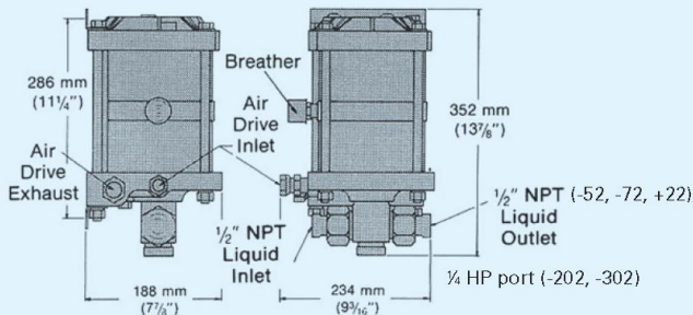
1.5 and 2 hp medium ratio pumps; -52, -72, -122, -202 and -302 ratios
