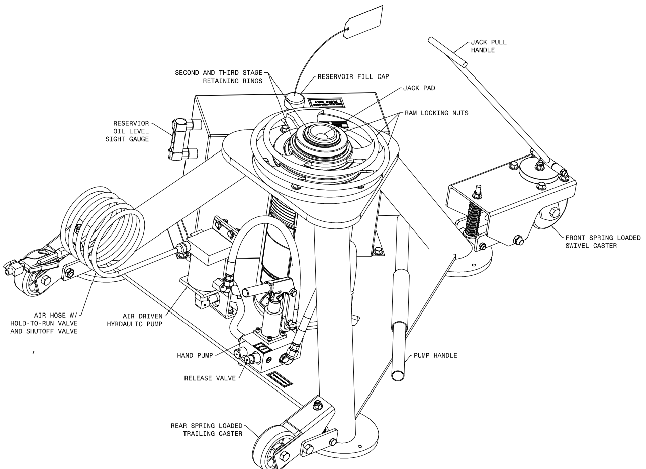
FIGURE 7.3 – Operator Controls
