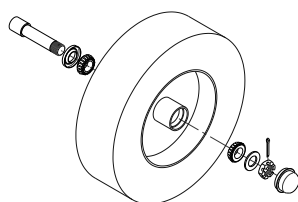
ITEM 10 DETAIL
