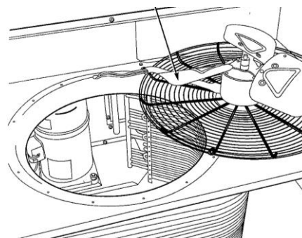
FIGURE 11 Condenser Coil Cleaning
