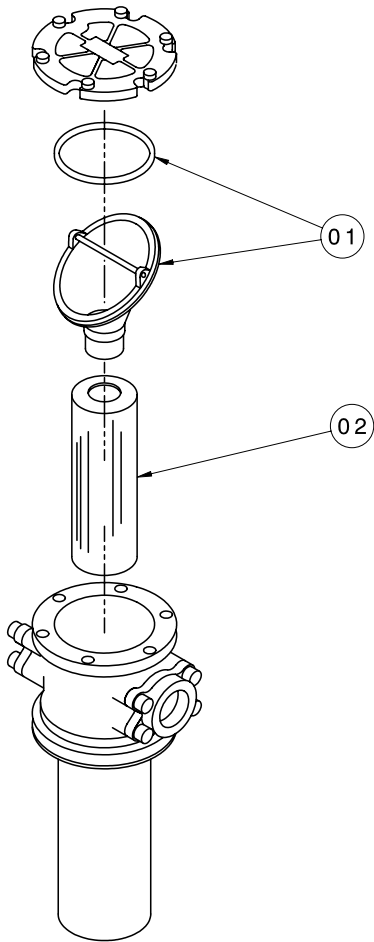
FIGURE 10.5.2 – Return Filter
