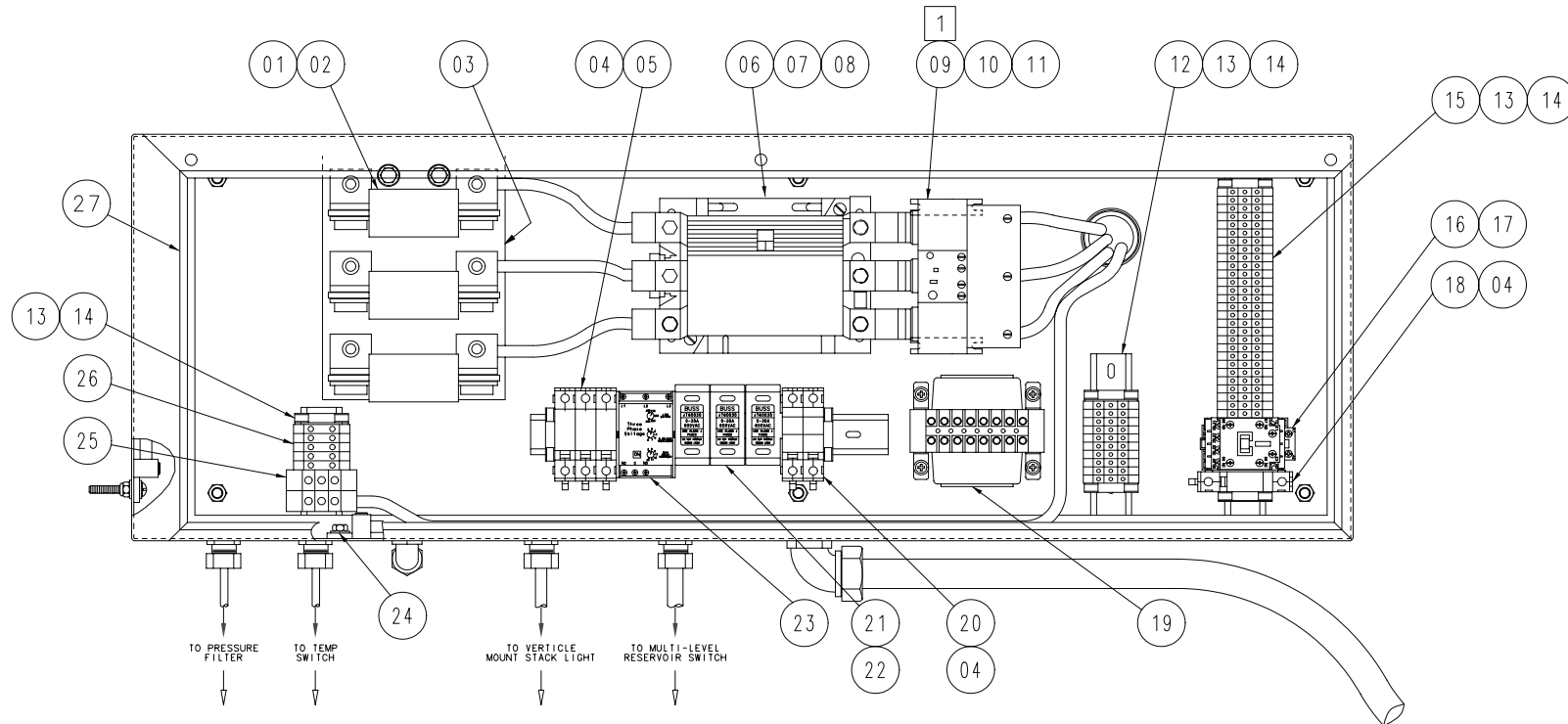
FIGURE 9.10 – Electrical Components
