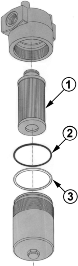
FIGURE 10.5.3 – Hand Pump (Option M) Filter
