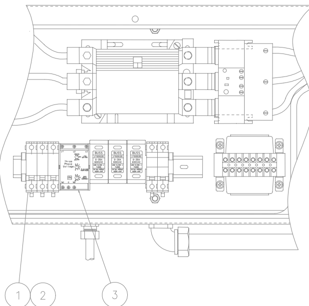
FIGURE 9.13.5 – Voltage/Phase Monitor
