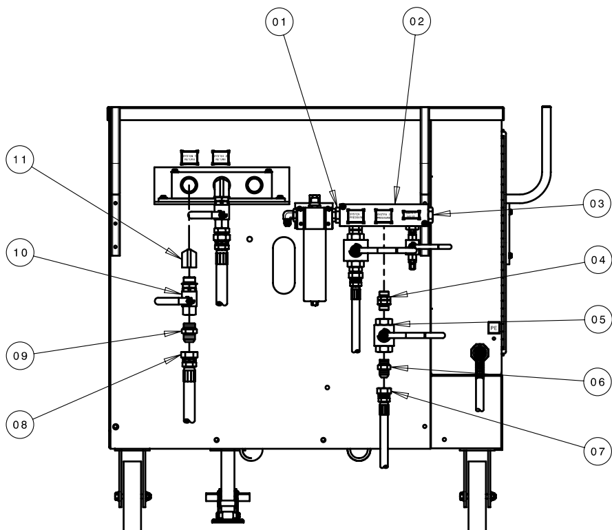
FIGURE 10.14.3 – Dual System
