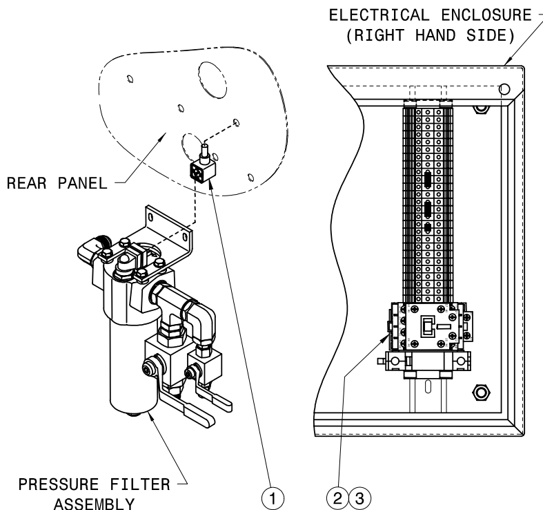
FIGURE 9.13.11 – Electric Filter Clogged Indicator
