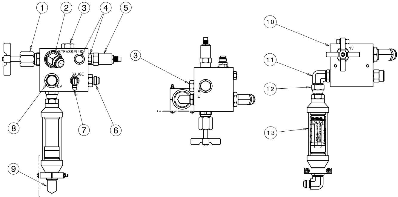
FIGURE 10.7.3 – Control Block/Flowmeter
