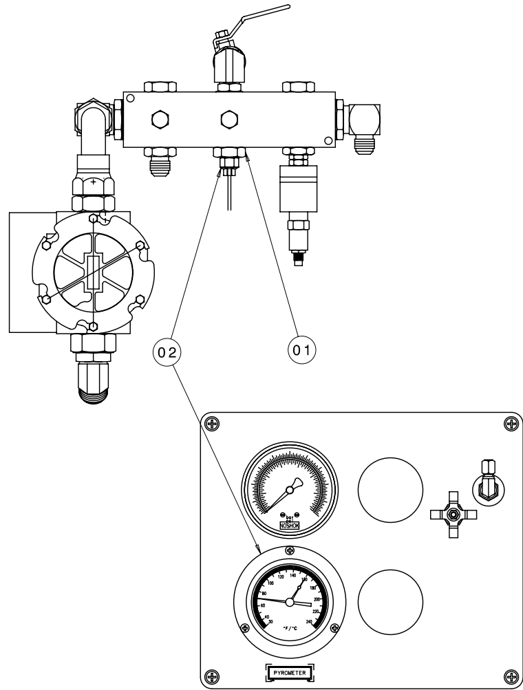
FIGURE 10.14.7 – Pyrometer
