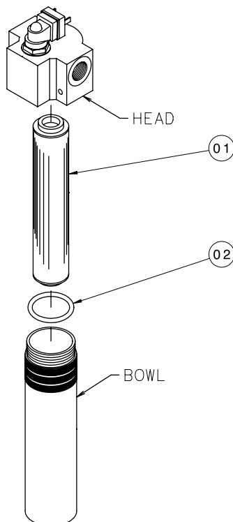
FIGURE 10.5.1 – Pressure Filter
