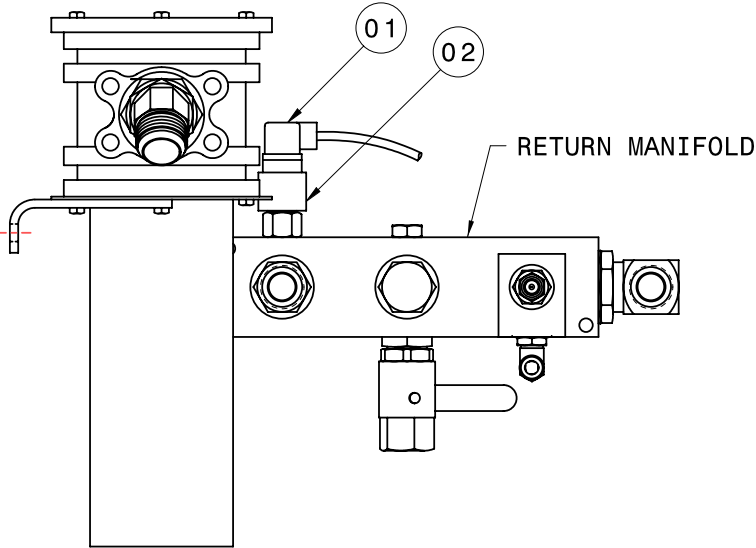
FIGURE 10.14.12 – Electric Over-Temperature
