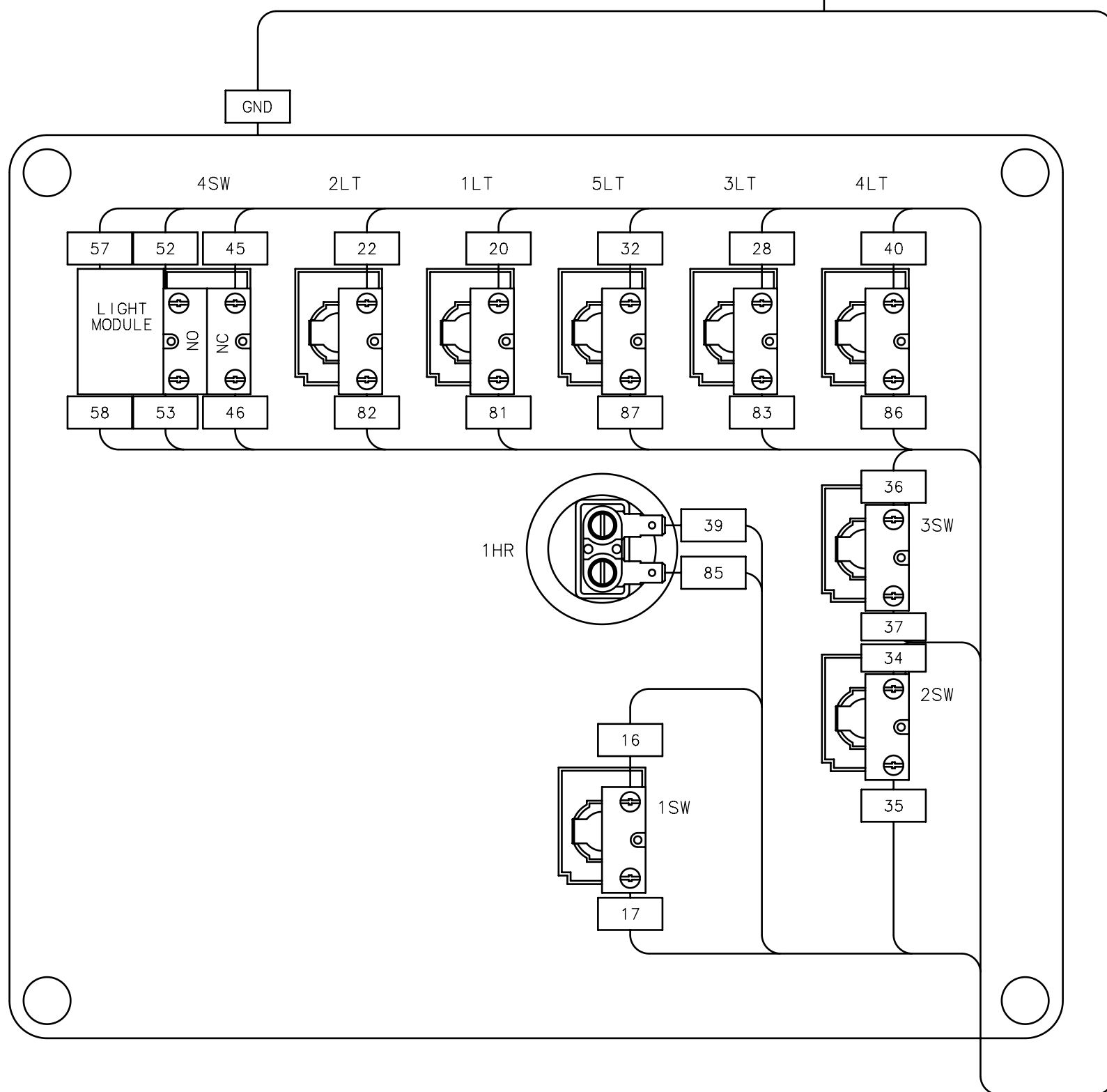
ELECTRICAL INSTRUMENT PANEL (LOOKING FROM REAR OF PANEL) SCALE: 9:16
