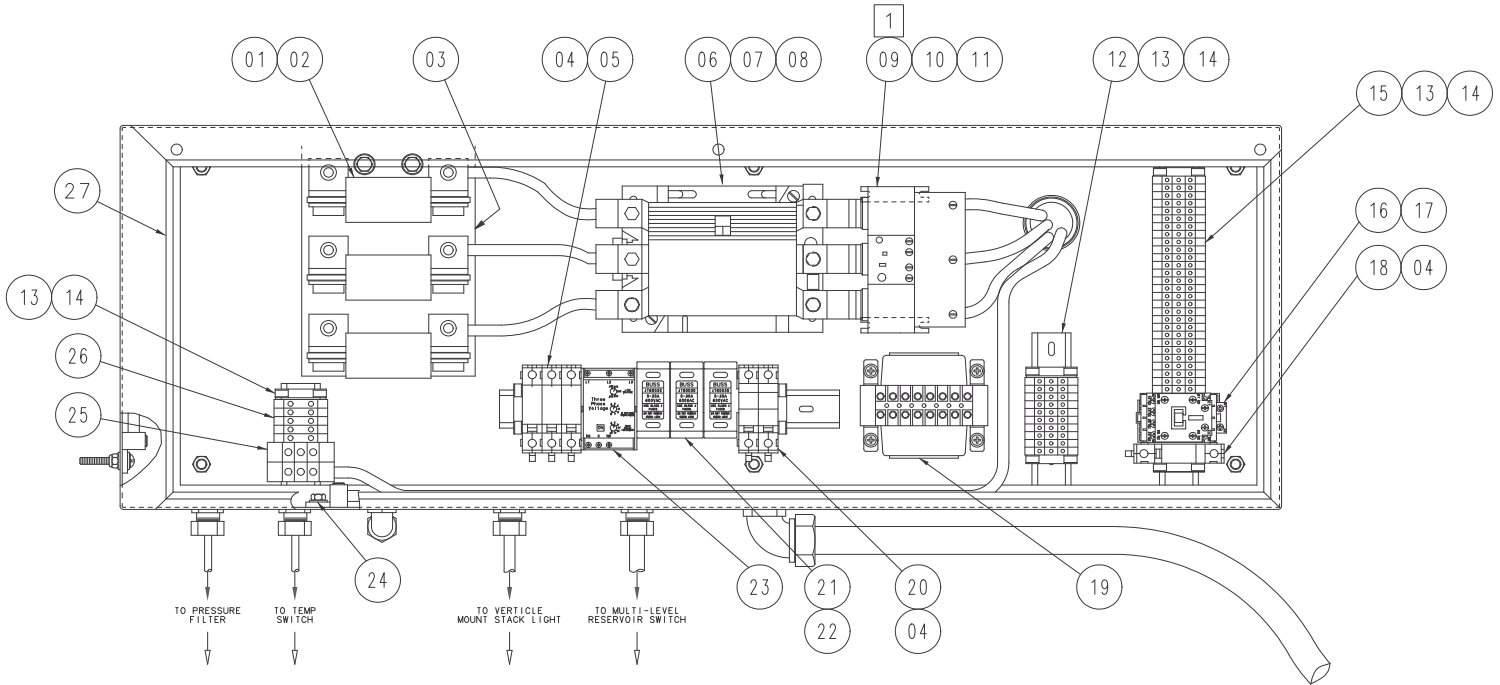
FIGURE 9.10 – Electrical Components
