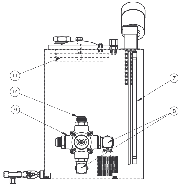
FIGURE 10.8 – Reservoir Assembly
