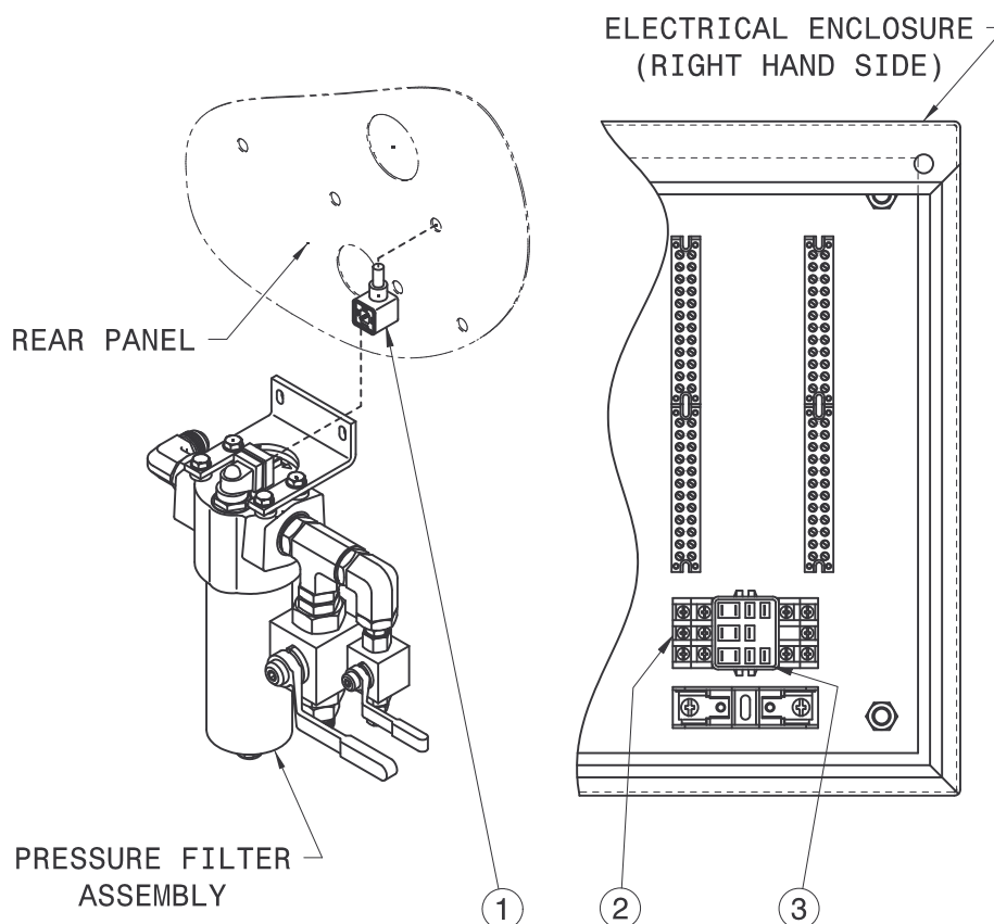
FIGURE 9.13.10 – Electric Filter Clogged Indicator
