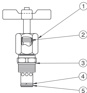
FIGURE 10.7.3.c – Bypass Valve
