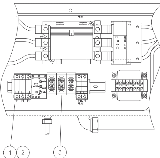
FIGURE 9.13.5 – Voltage/Phase Monitor
