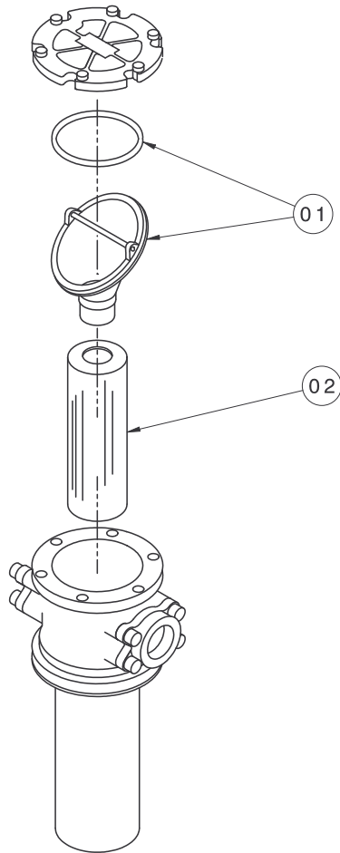
FIGURE 10.5.2 – Return Filter
