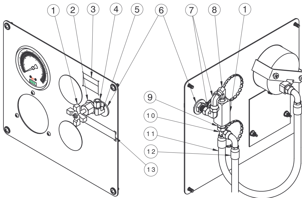
FIGURE 10.14.9 – Calibration Port
