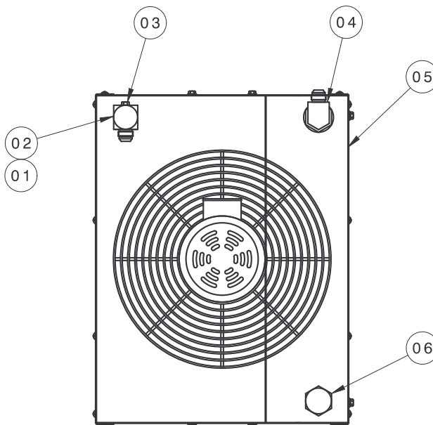
FIGURE 10.12 – Heat Exchanger Assembly
