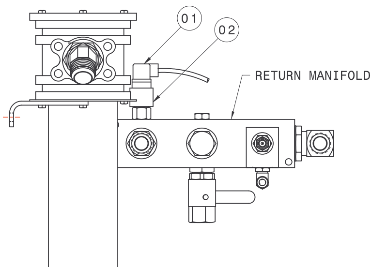
FIGURE 10.14.11 – Electric Over-Temperature
