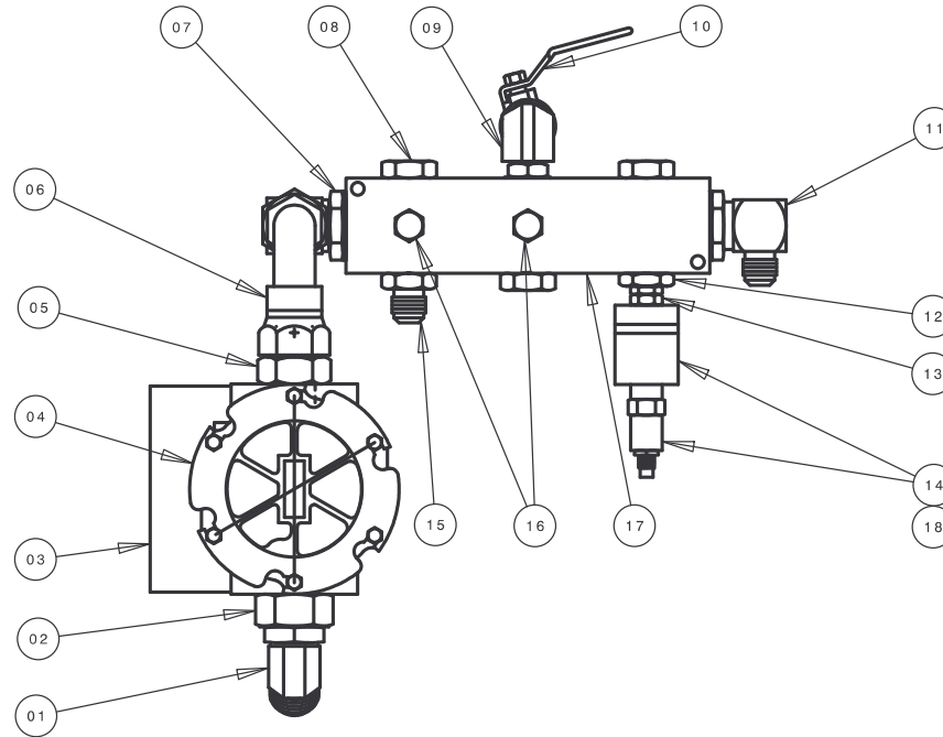
FIGURE 10.9 – Return Manifold Assembly PARTS LIST
