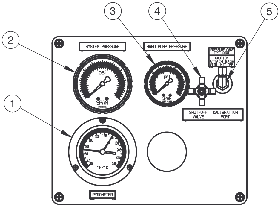
FIGURE 10.7.2 – Hydraulic Panel
