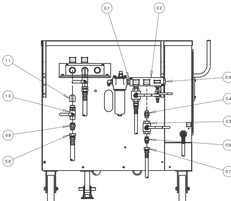
FIGURE 10.14.2 – Dual System
