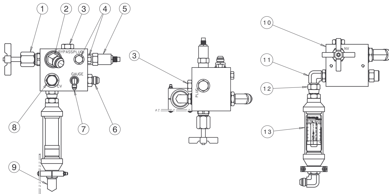
FIGURE 10.7.3 – Control Block/Flowmeter
