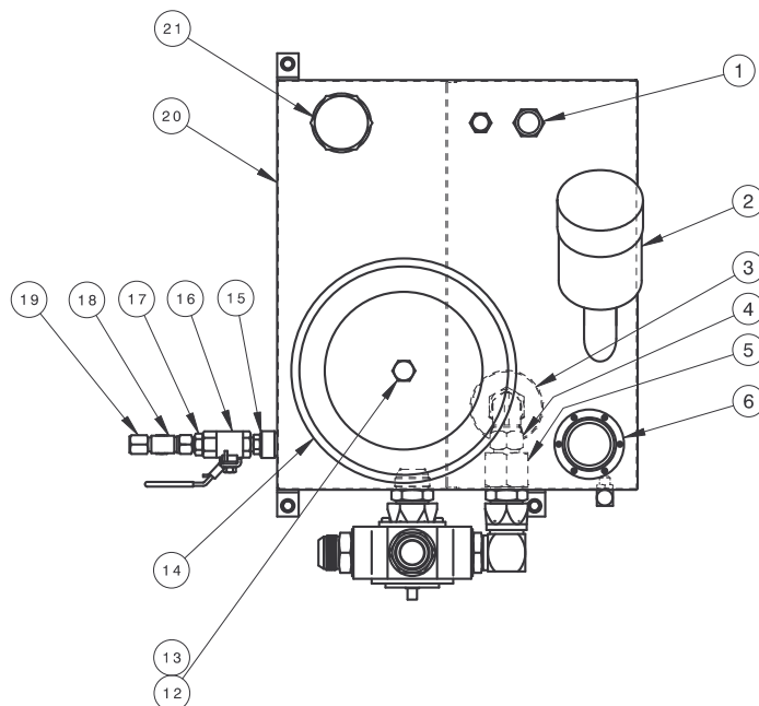
FIGURE 10.8 – Reservoir Assembly
