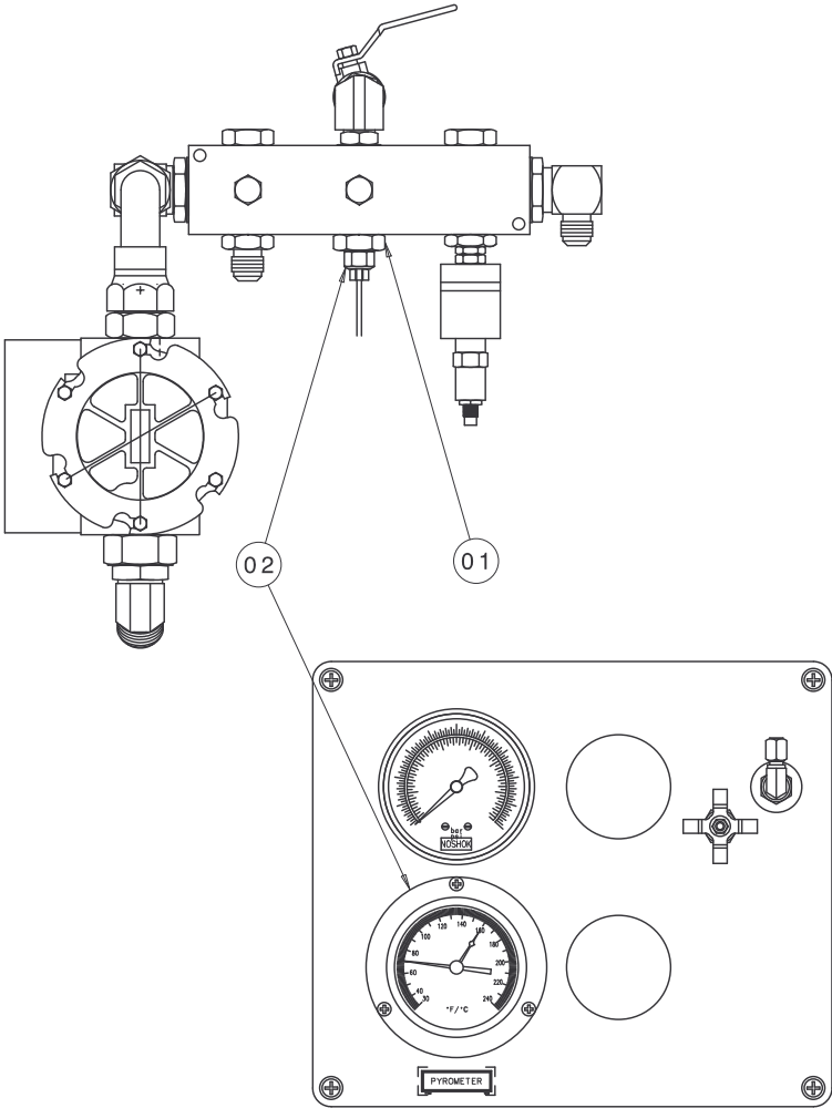
FIGURE 10.14.6 – Pyrometer
