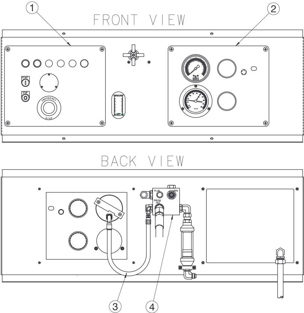
FIGURE 10.7 – Instrument Panel
