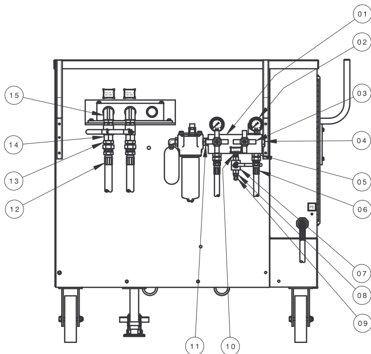
FIGURE 10.14.3 – Crossover Check
