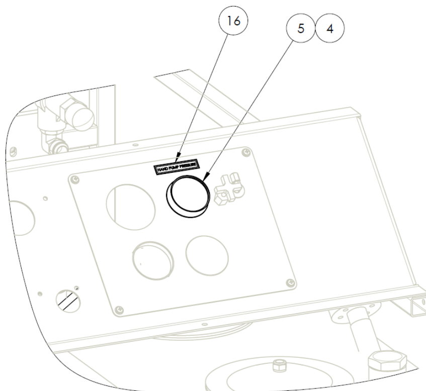
PRESSURE GAUGE
