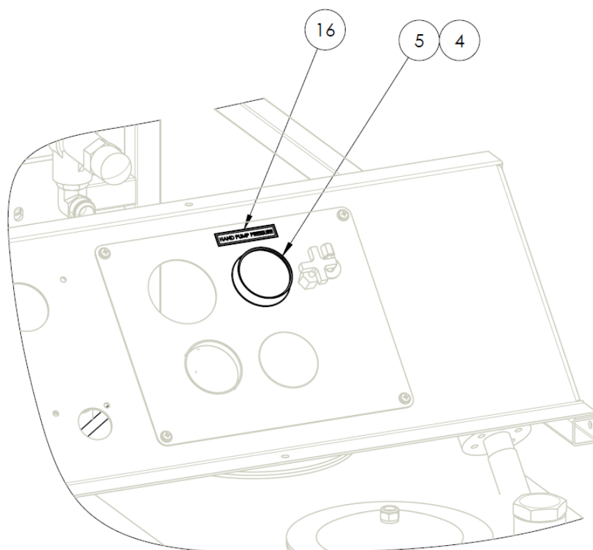
PRESSURE GAUGE
