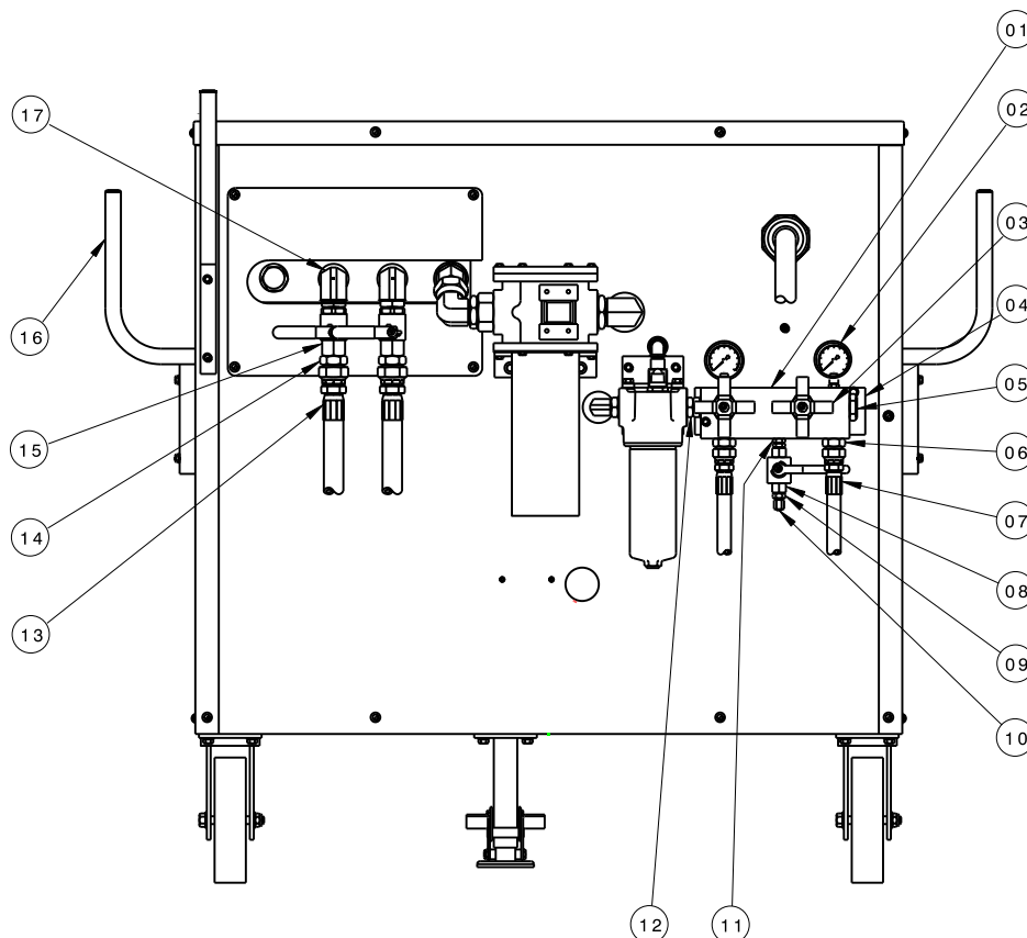
Model 5J11 & 5J21 Parts List Fluid Type: MIL-PRF-5606 & MIL-PRF-83282
