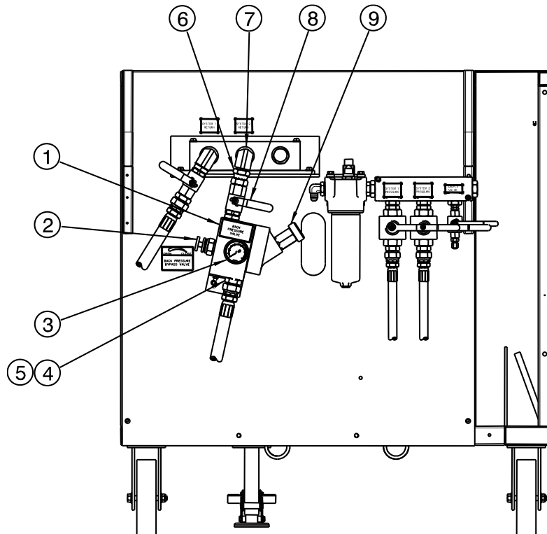
Model 5J11 & 5J21 Parts List Fluid Type: MIL-PRF-5606 & MIL-PRF-83282
