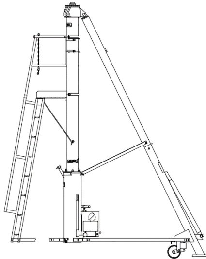
Model: 8802 Single Stage Fixed Height Hydro – Mechanical Aviation Tripod jack
