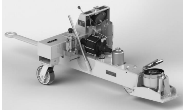
Model: 8899 Two Stage Hydraulic Aviation Floating Auto-Retract Axle Jack S/N 256 and Up S/N 13000 and Up S/N 5610191201 and Up
