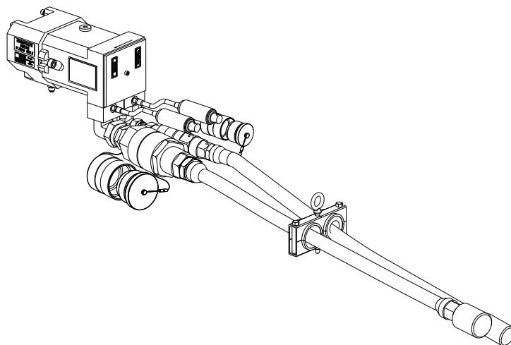
Model: AGE17080A Ground Test Tool Airbus A350 Ram Air Turbine
