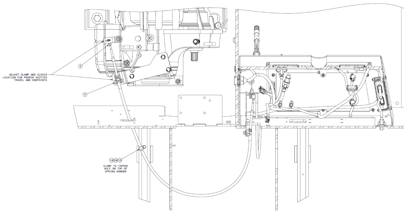
SECTION D-D SHIFT CABLE ROUTING
