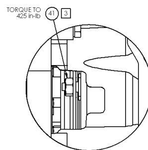
DETAIL C SCALE 2 : 3
